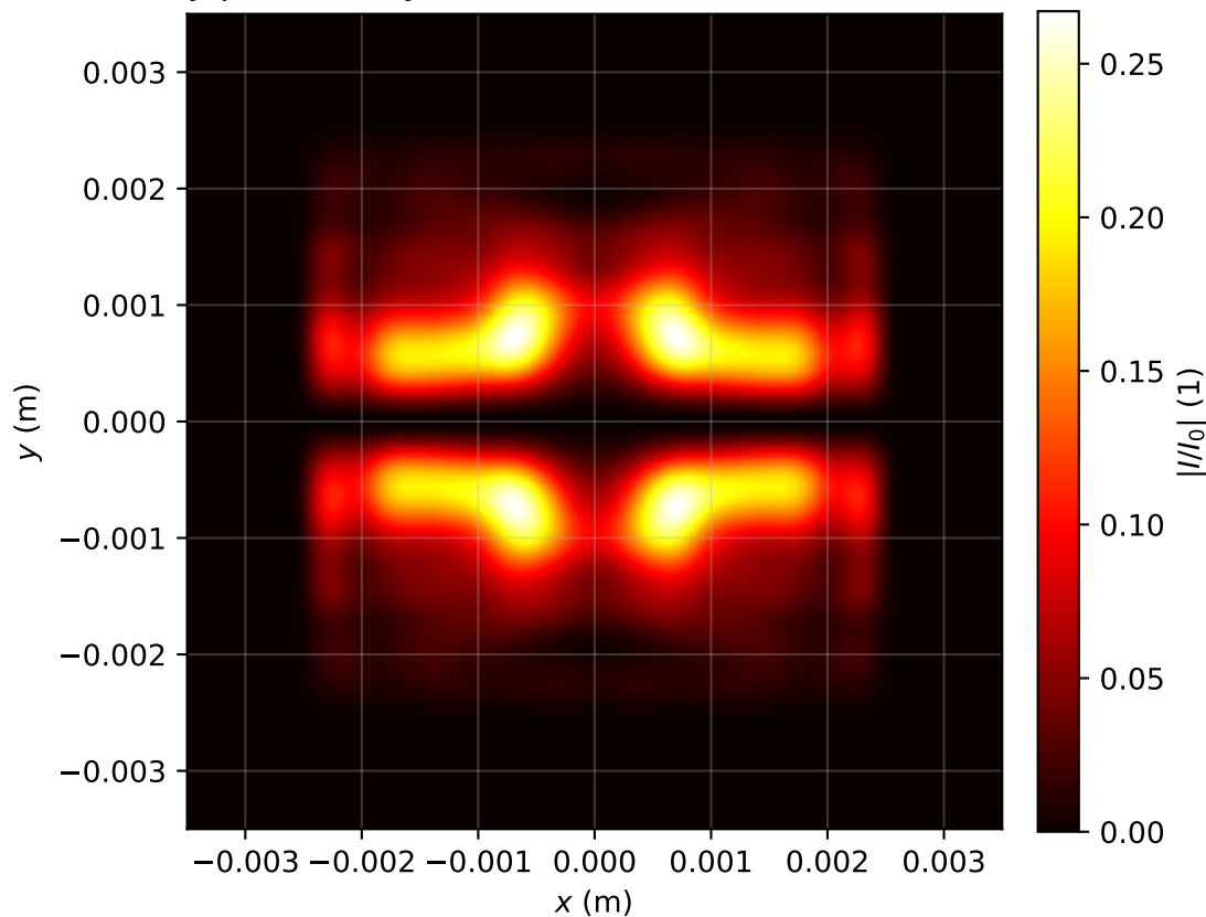
Intensity profile I(x, y, z = 3.901)/I_0 , P_{in}=4.0P_{cr} , artificial time
